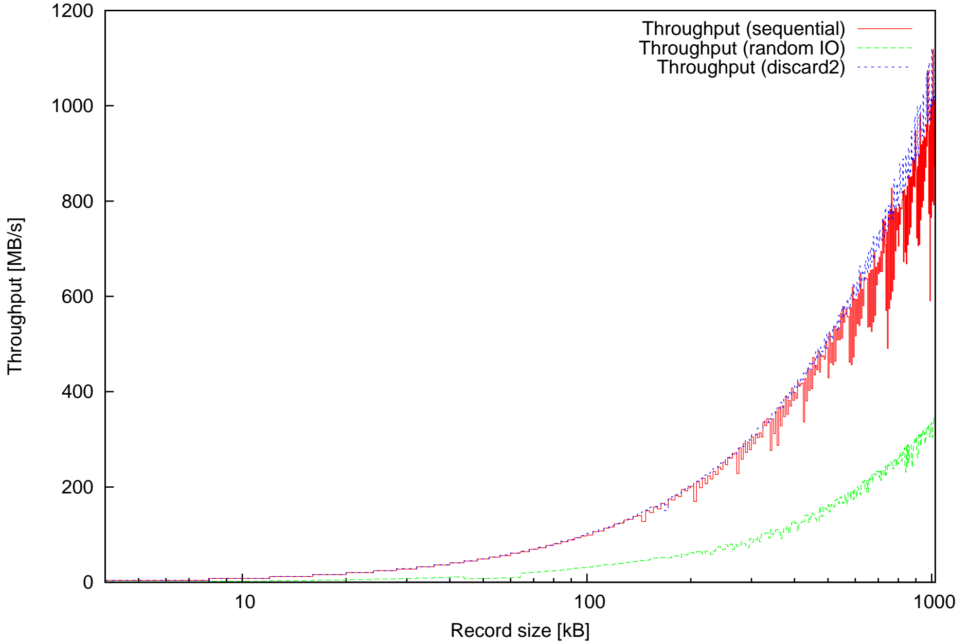
Comparison of Throughput in sequential and Random IO mode
