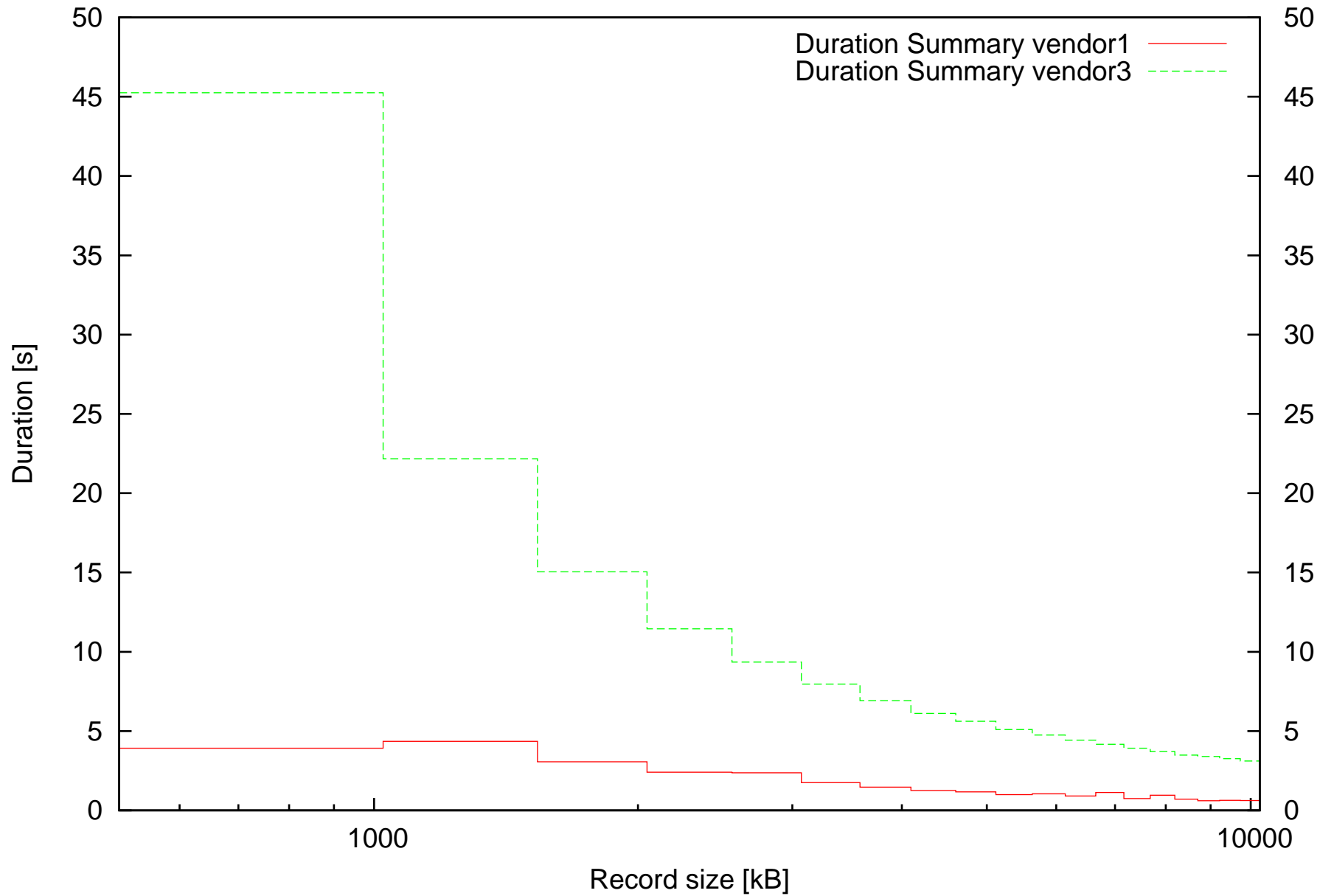
Summary of duration of discard operations depending on record size
