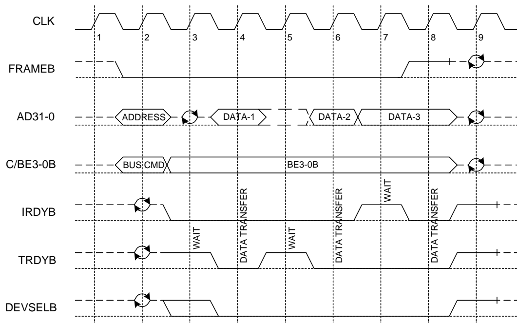
Figure 23. Memory Read below 4GB (32-bit address, 32-bit data; 32-bit slot)
