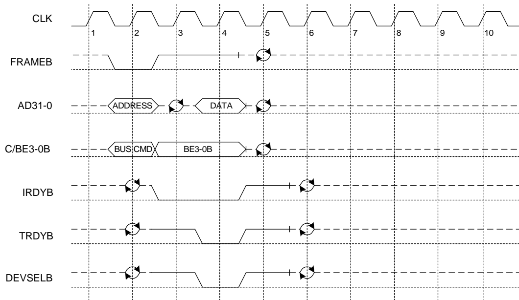
Figure 18. I/O Read
