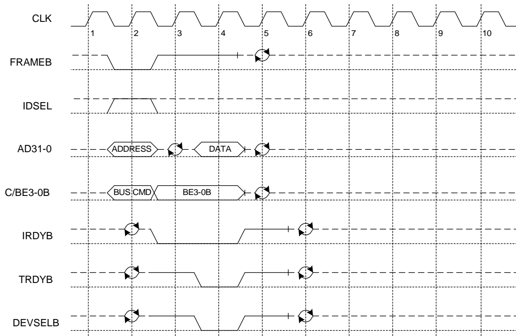
Figure 20. Configuration Read
