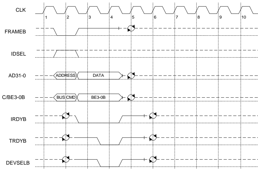
Figure 21. Configuration Write
