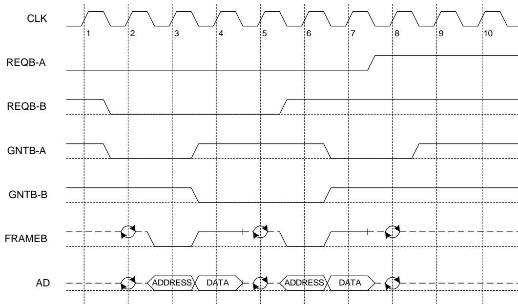
Figure 22. Bus Arbitration
