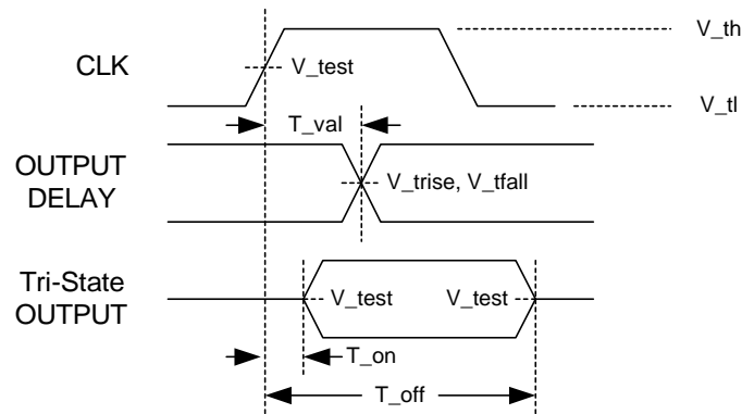
Figure 14. Output Timing Measurement Conditions
