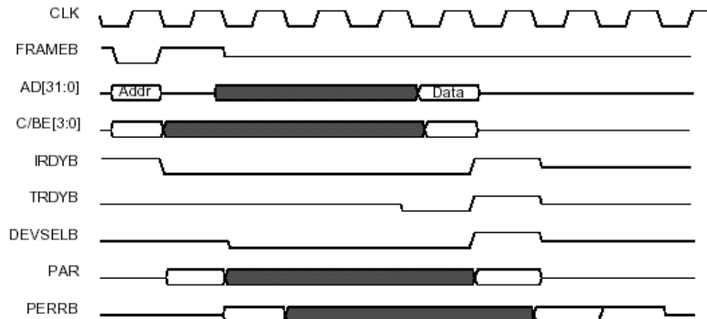
Figure 5. Target Read Operation
