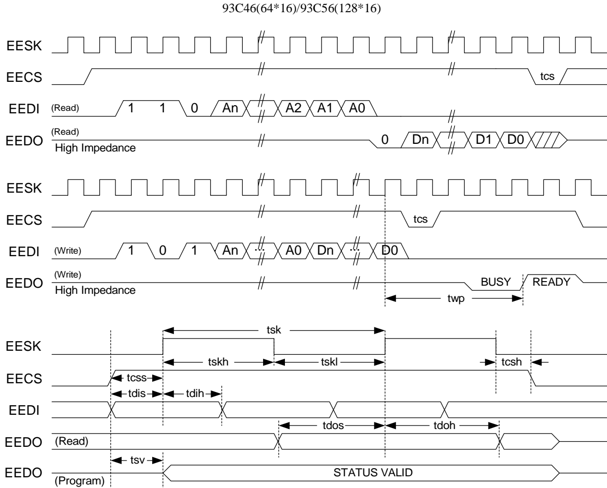
Figure 13. Serial EEPROM Interface Timing
