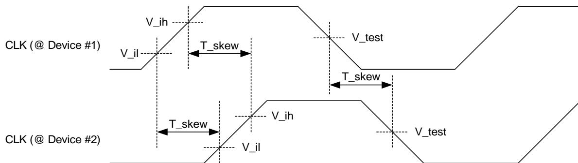
Figure 17. Clock Skew Diagram
