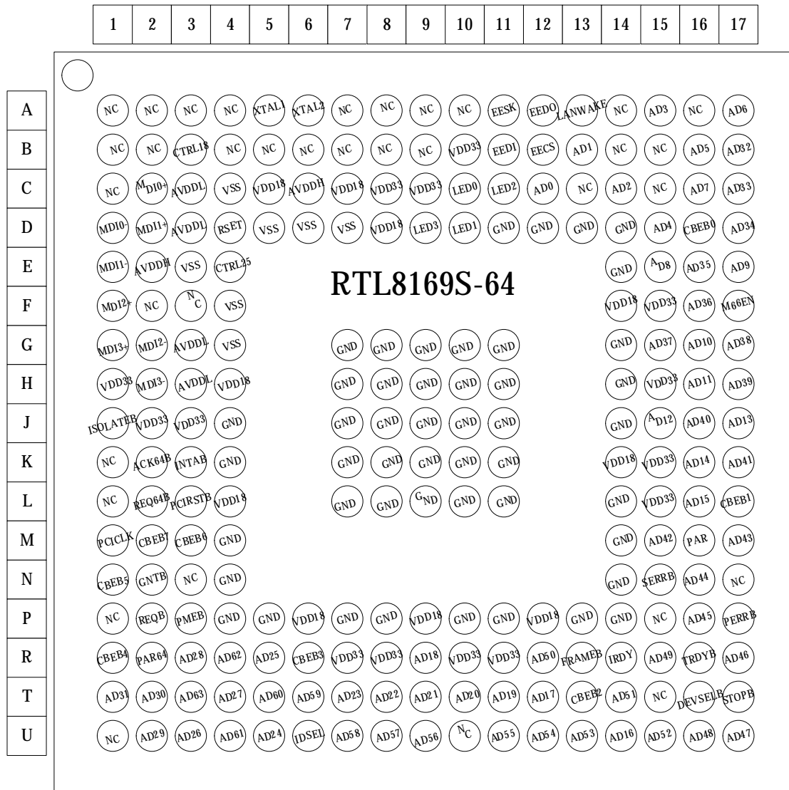
Figure 2. RTL8169S-64 233-Pin TFBGA Pin Assignments
